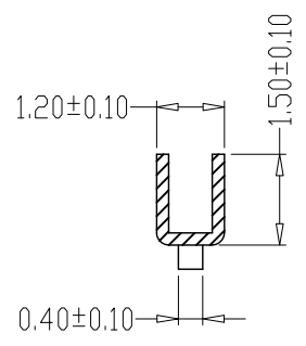
SEC:C-C
